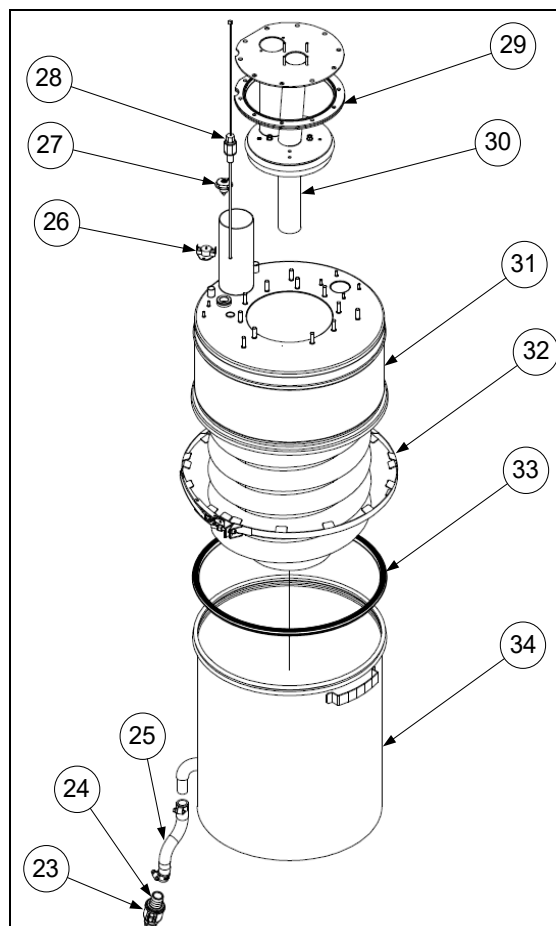
Illustration 53 - Evaporation Chamber Assembly Exploded View
