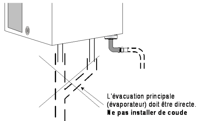
(Illus. 8b) Installation non recommandée
