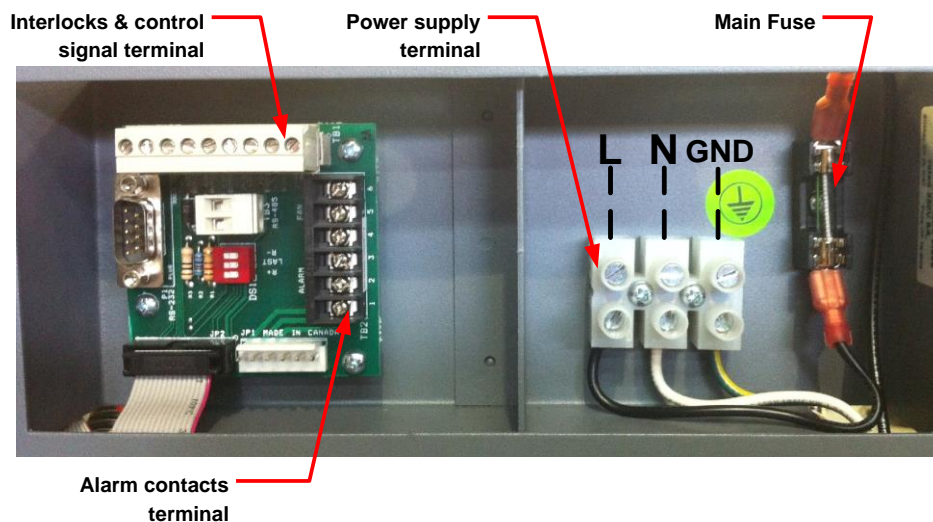
Electrical connection - Fig. 40
