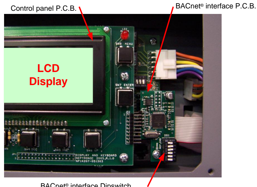
Location of BACnet interface dip switch - Fig. 48
