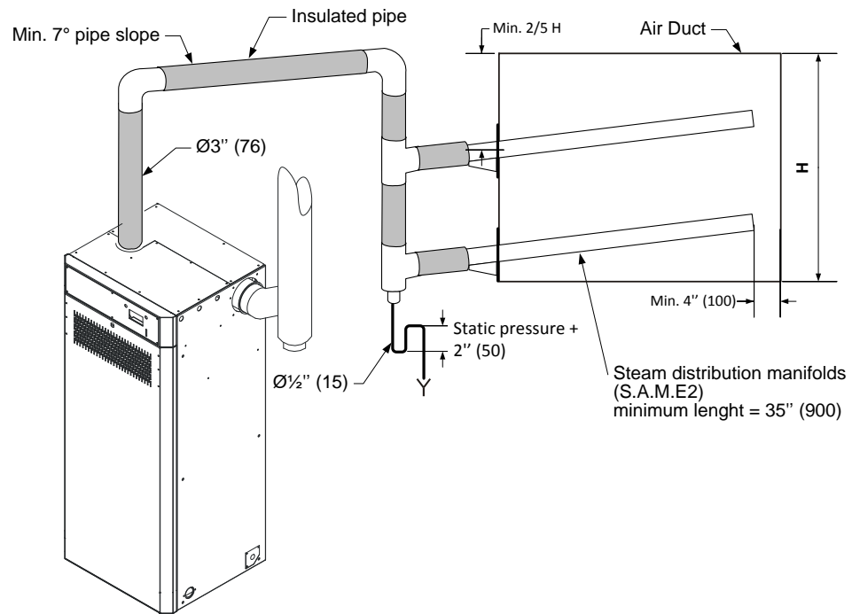
Steam pipe work SKG3-110, SAM - Fig. 22 (dimensions in bracket are in mm)
