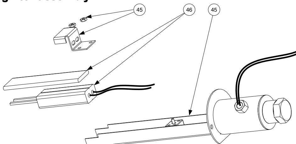
Igniter assembly - Fig. 54
