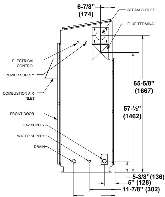
Weather proof enclosure. Connection positions 1 to 3 modules- Fig. 7 (dimensions in bracket are in mm)
