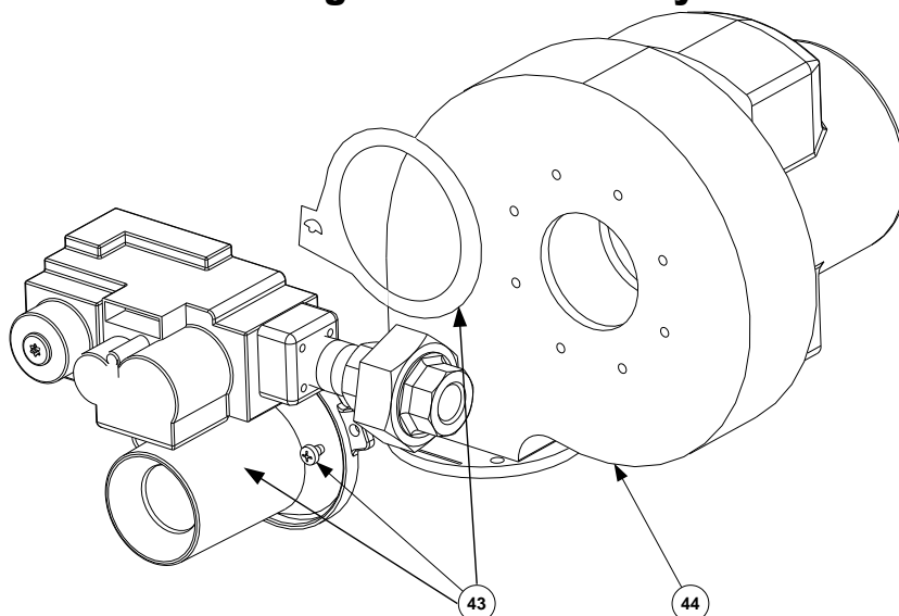
Combustion blower and gas valve assembly - Fig. 53
