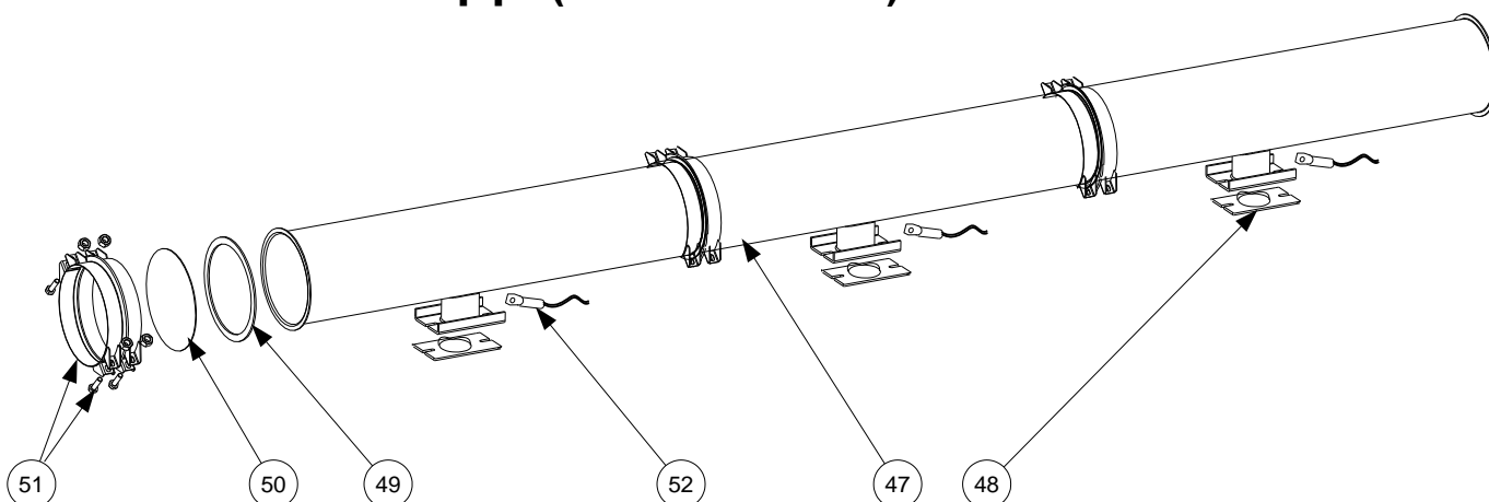
Flue pipe assembly - Fig. 55
