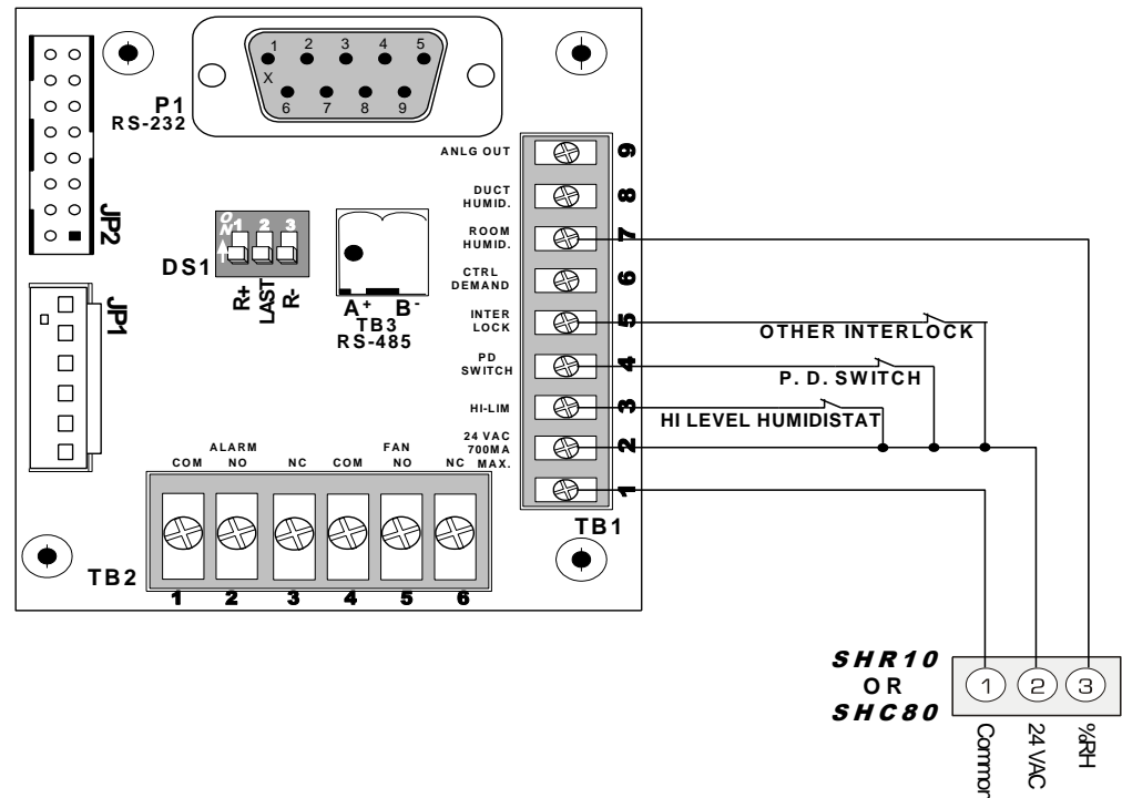
Humidity signal from humidity sensors - Fig. 44
