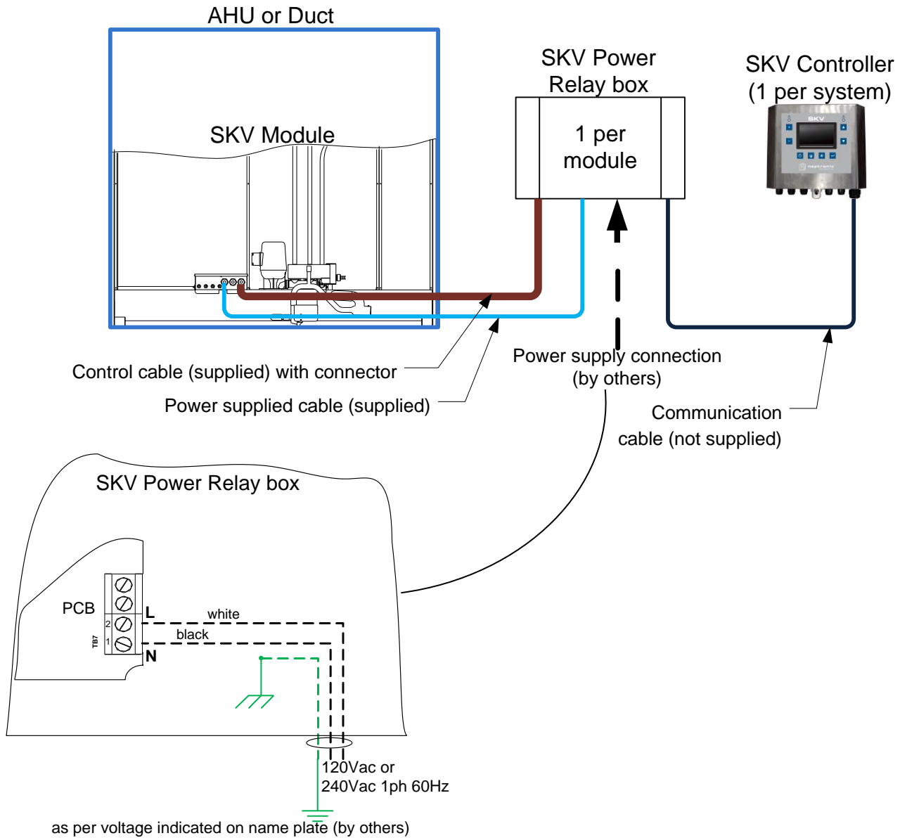
Illustration 12 - Power Supply Connections
