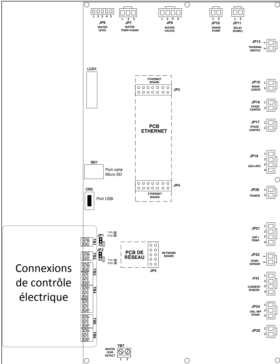
Illustration 42 - Circuit imprimé
