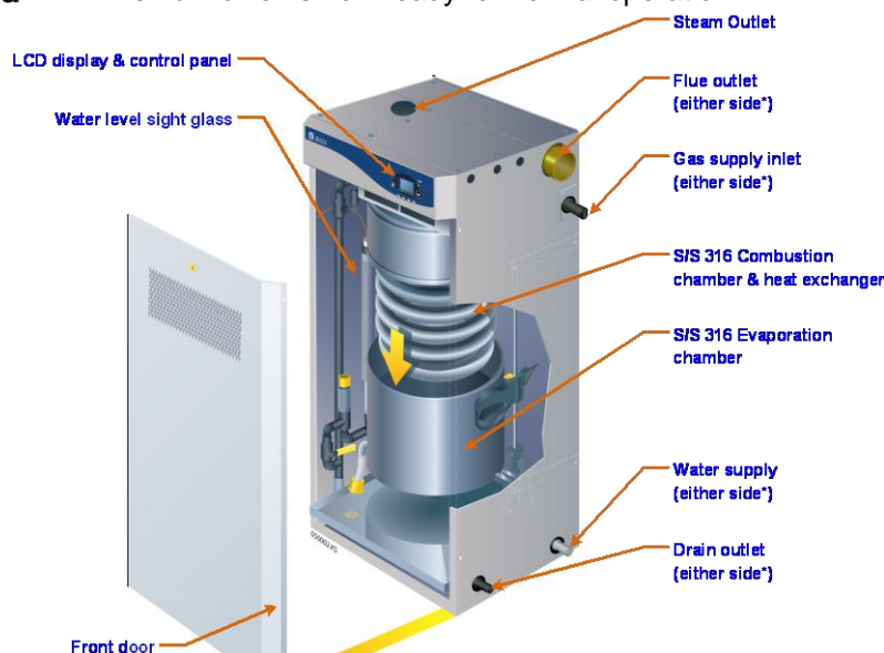
General overview reminder - Fig. 51
