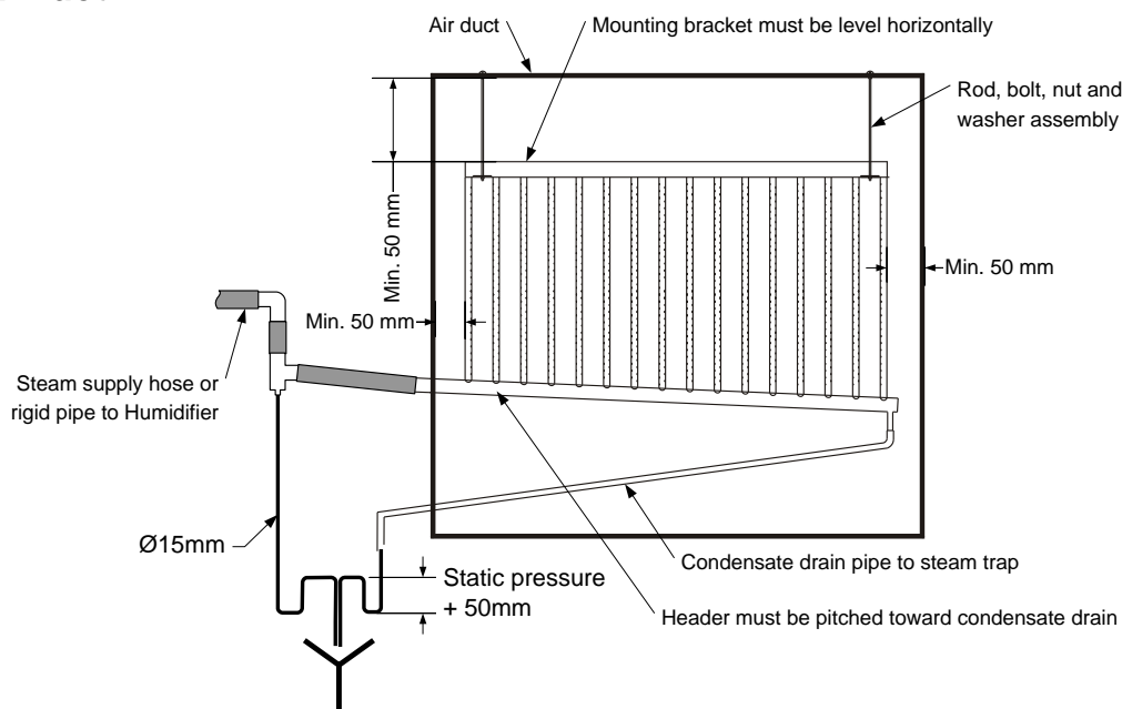
Multi-Steam in horizontal duct - Fig. 24
