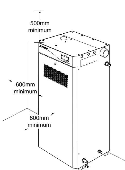
Standard enclosure clearances - Fig. 12
