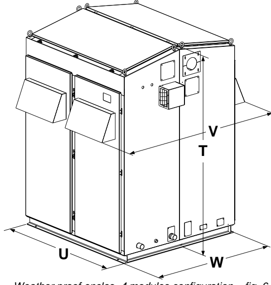
Weather proof enclos. 4 modules configuration – fig. 6
