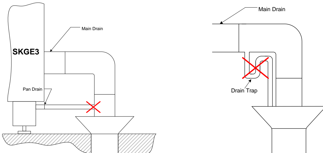
Drain connection: Incorrect installation - Fig. 33
