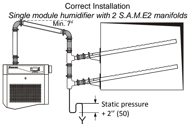
Steam distribution correct installation 2 - Fig. 15b (dimensions in bracket are in mm)
