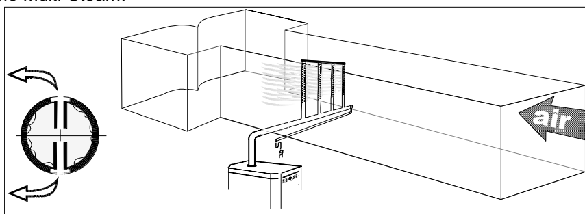
Illustration 16 - Système Multi-Steam
