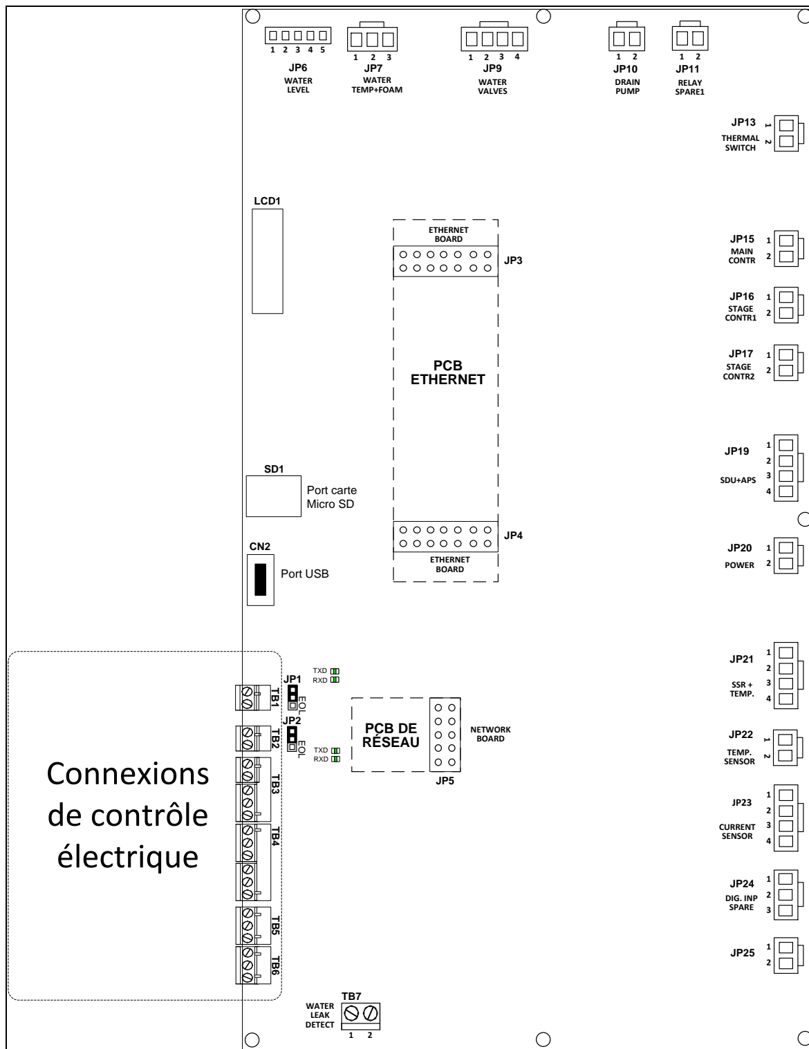
Illustration 42 - Circuit imprimé
