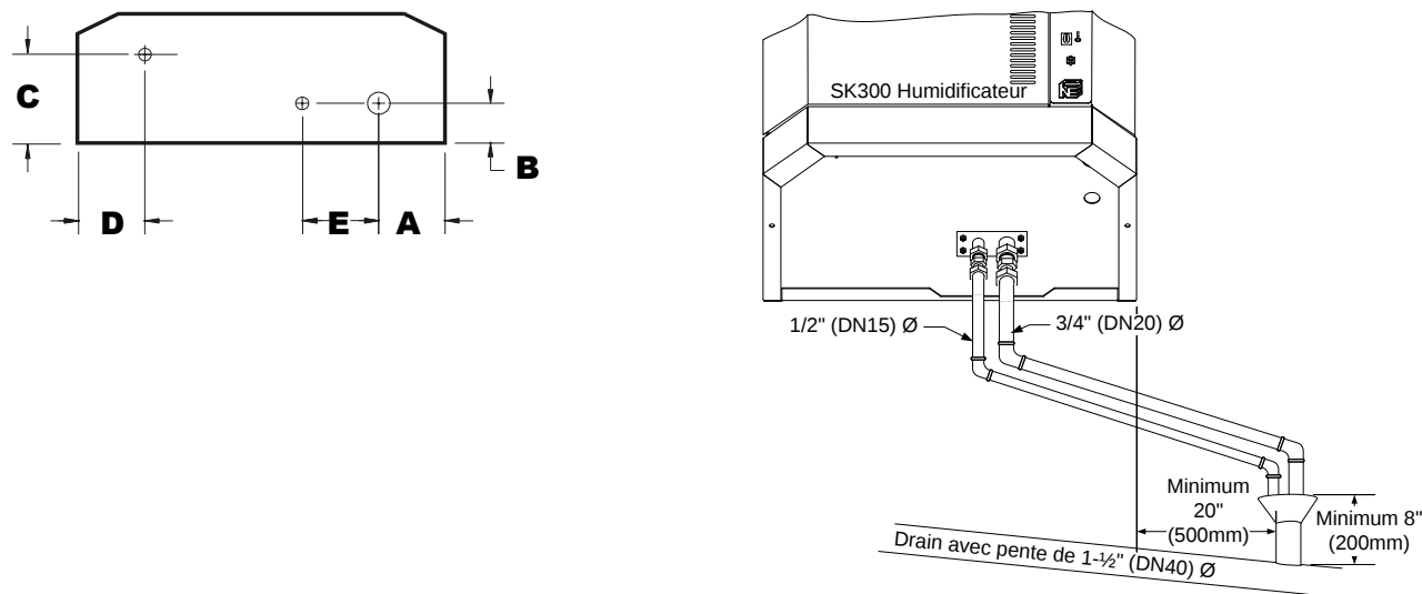
Illustration 21 - Raccordement de plomberie
