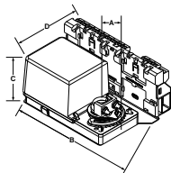
EVC with a built-in 70 in. lb. Actuator
