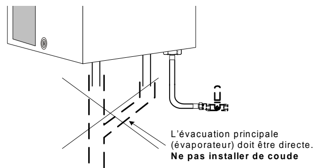
(Illus. 10b) Installation non recommandée
